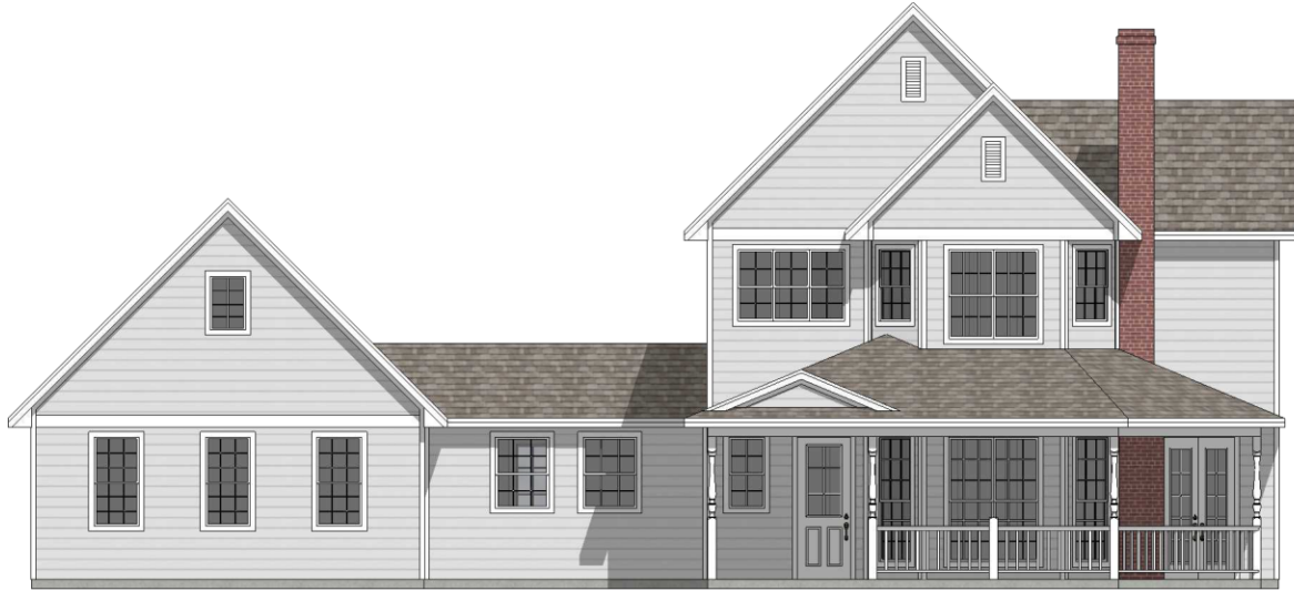
Front Elevation
